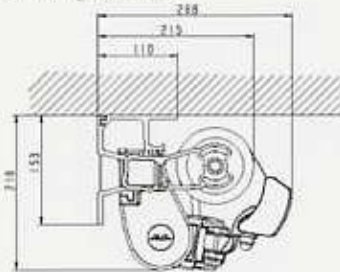
Nova Classic, ceiling-mounted
