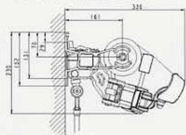
Nova Marcesa Flexi, wall-mounted
