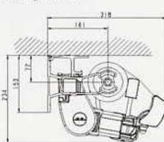
Nova Marcesa, ceiling-mounted
