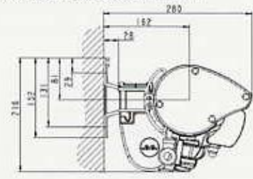
Nova Classic Cassette, wall-mounted
