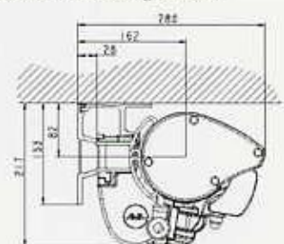
Nova Classic Cassette, ceiling-mounted
