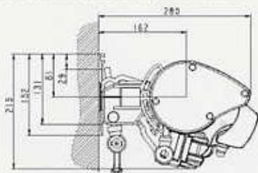
Nova Classic Flexi Cassette, wall-mounted
