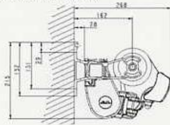
Nova Classic, wall-mounted
