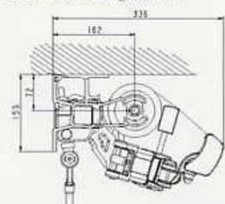
Nova Marcesa Flexi, ceiling-mounted
