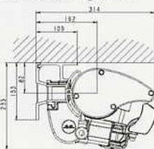
Nova Marcesa Cassette, ceiling-mounted
