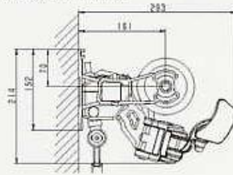
Nova Classic Flexi, wall-mounted
