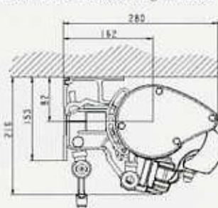
Nova Classic Flexi Cassette, ceiling-mounted
