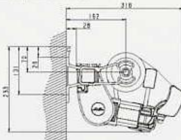
Nova Marcesa, wall-mounted
