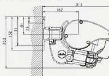
Nova Marcesa Cassette, wall-mounted
